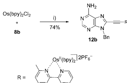
Scheme 6. Synthesis of the Os II complex: i) 1. ethylene glycol, 150 °C, 2 h; 2. saturated aqueous solution of NH 4 PF 6 .
