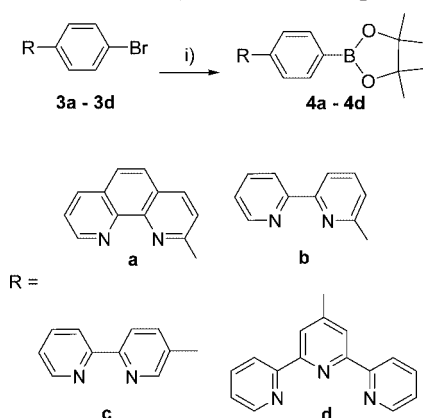
Scheme 2. Synthesis of the ligands: i) bis(pinacolatodiboron) (1.2 equiv.), [\text{Pd}(\text{dppf})\text{Cl}_2] (5 mol-%), KOAc (1.5 equiv.), dioxane, 80 °C.
