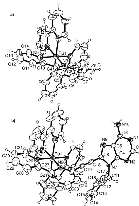
Figure 1. ORTEP diagram of 5b (a) and 10b (b) (thermal ellipsoids drawn at the 30% probability level).
