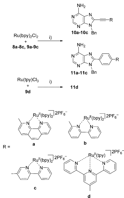
Scheme 5. Complexations of the conjugates: i) 1. ethylene glycol, 150 °C, 2 h; 2. saturated aqueous solution of NH 4 PF 6 .
