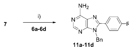
Scheme 7. Cross coupling reactions with complexes. i) [Pd(OAc) 2 ] (10 mol-%), P(Ph-SO 3 Na) 3 (50 mol-%), Cs 2 CO 3 (3 equiv.), CH 3 CN/H 2 O (1:1).
