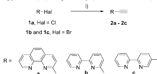
Scheme 1. Synthesis of the ligands: i) 1. [Pd(PPh 3 ) 2 Cl 2 ] (5–10 mol-%), CuI (10 mol-%), TMSA (2.2 equiv.), Et 3 N (3.2 equiv.), DMF or THF, 60–70 °C; 2. MeOH/THF KF (2 equiv.).
