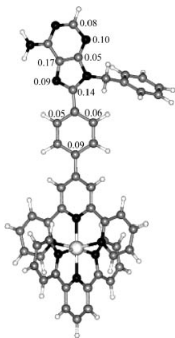
Figure 3. The equilibrium geometry of 11d . Denoted are the calculated spin densities for the oxidized \text{Ru}^{\text{III}} complex demonstrating that the unpaired electron is localized on the adenine moiety rather than on the Ru atom.
