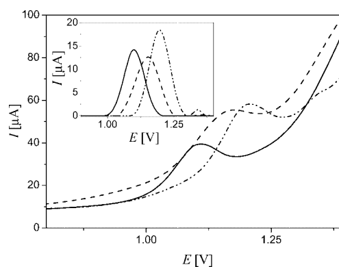
Figure 2. Sections of square-wave voltammograms of unsubstituted complex [\text{Ru}(\text{bipy})_3]^{2+} (solid), compound 5b (dash) and compound 10b (dash-dot-dot) measured at the CPE. Inset shows the same voltammograms after baseline subtraction.
