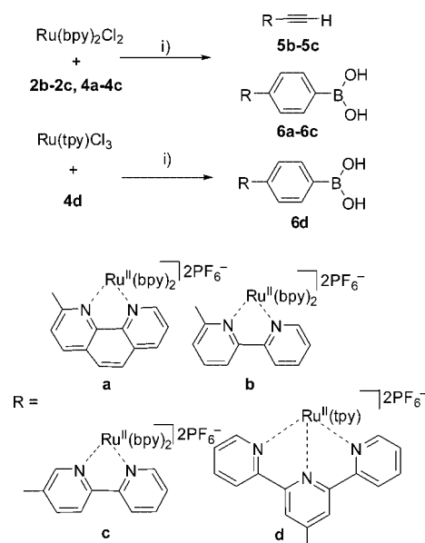
Scheme 3. Complexation reactions: i) 1. ethylene glycol, 150 °C, 2 h; 2. saturated aqueous solution of \text{NH}_4\text{PF}_6 .
